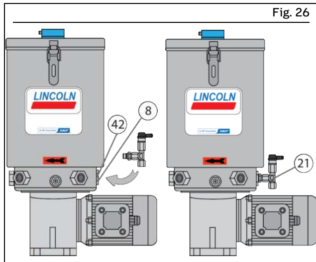
Installing the pressure limiting valve
