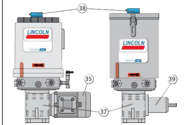
Main components
