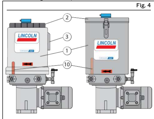
Main components
