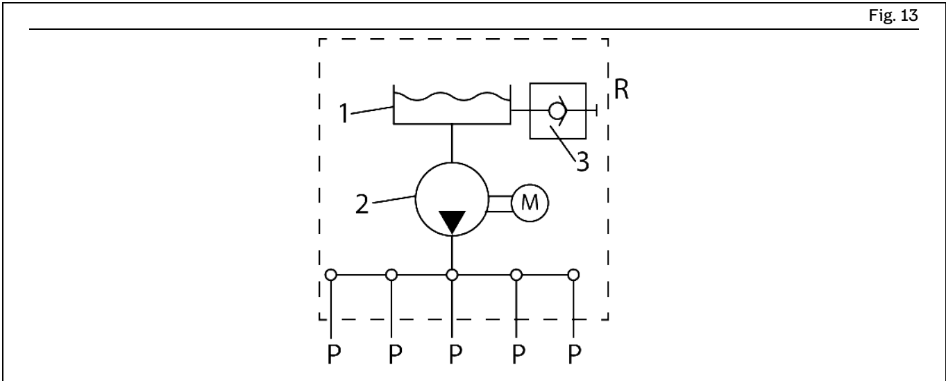
Hydraulic connection diagram for P205
